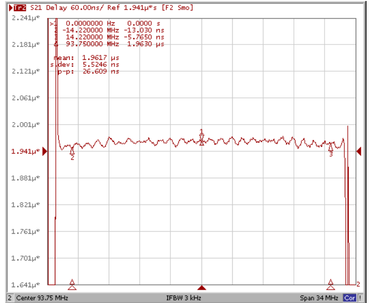
Group Delay Variation F_o \pm 14.22\text{MHz}
