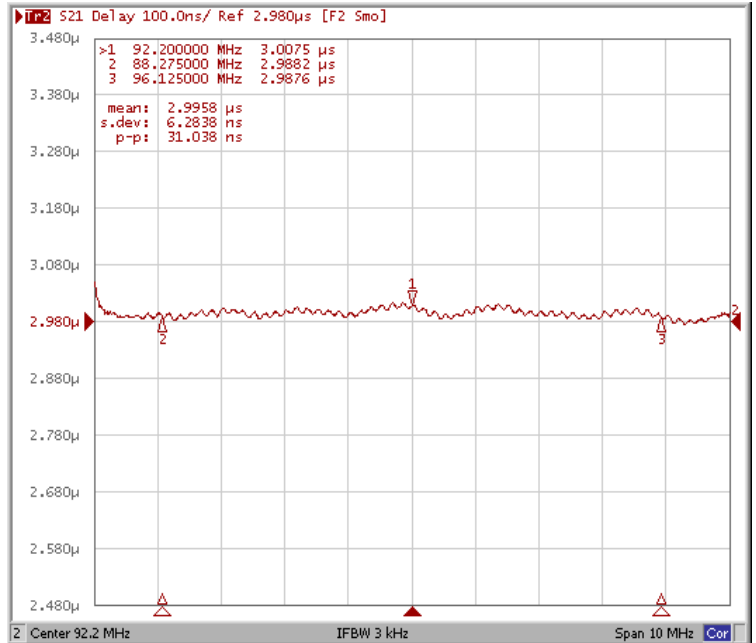
Group Delay Variation Fo±3.925MHz
