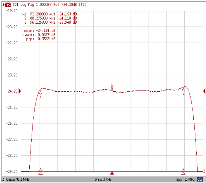
Ripple Variation Fo±3.925MHz
