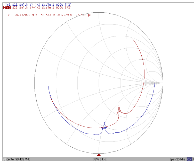
Smith Chart
