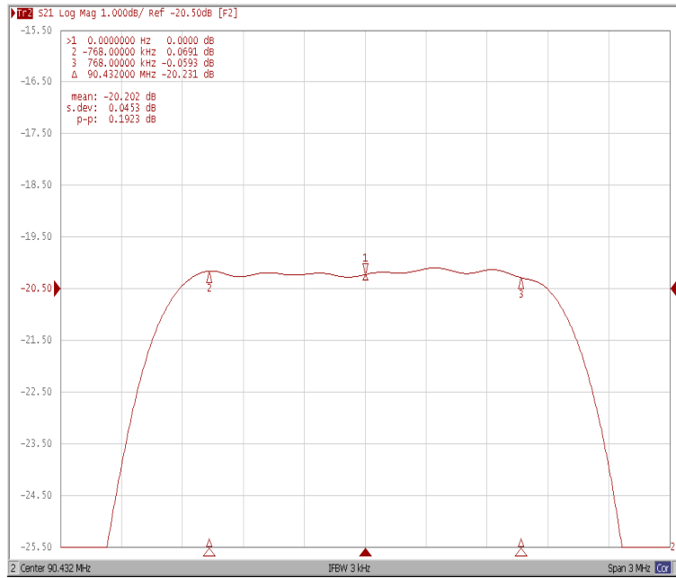
Ripple Variation Fo \pm 0.768\text{MHz}
