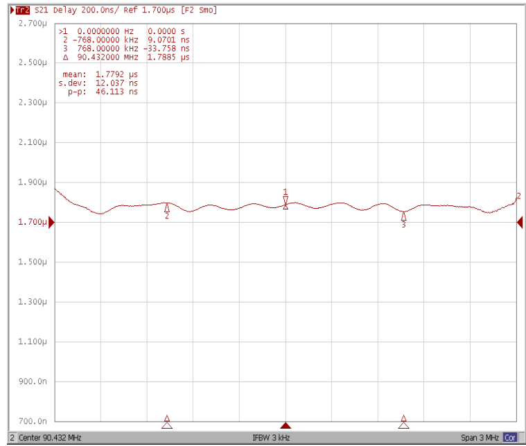
Group Delay Variation Fo \pm 0.768\text{MHz}
