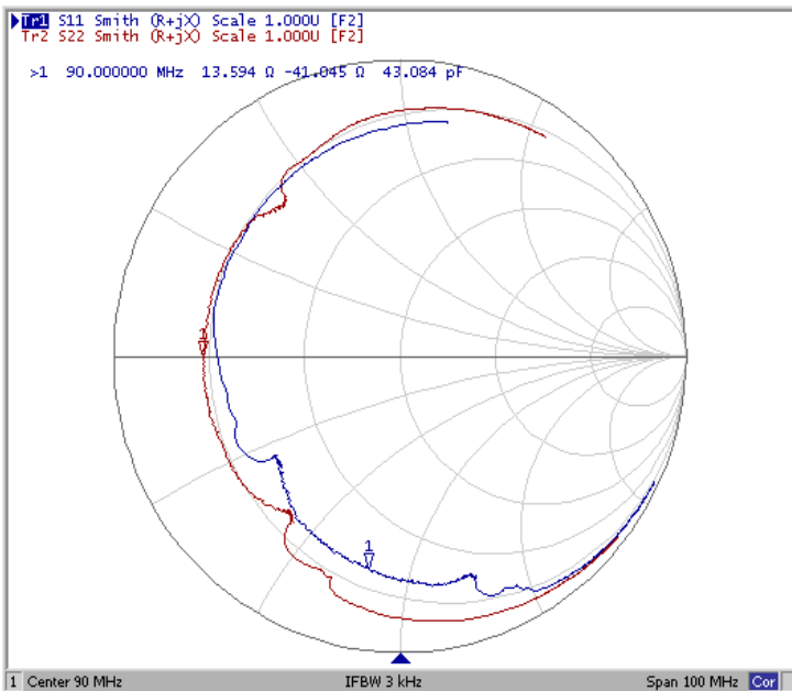
Smith Chart
