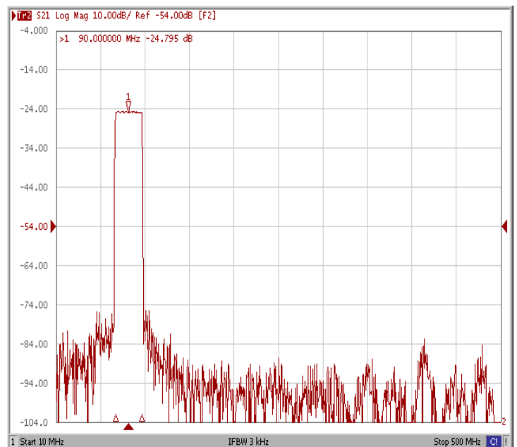
Wide Band
