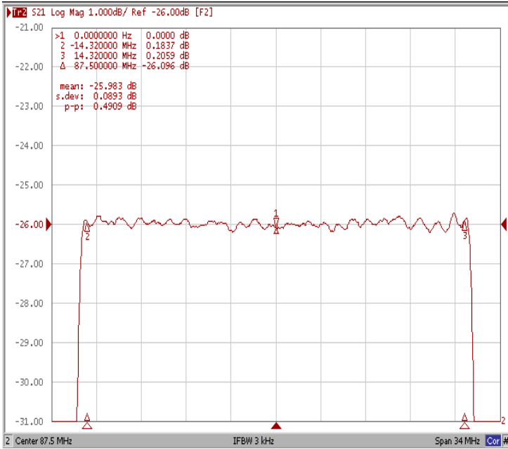
Ripple Variation F_o \pm 14.32\text{MHz}
