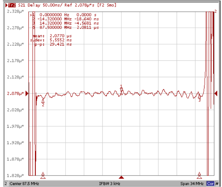
Group Delay Variation F_o \pm 14.32\text{MHz}
