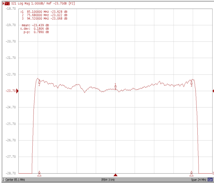
Ripple Variation F_o \pm 9.42\text{MHz}
