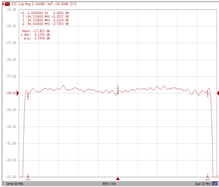
Ripple Variation F_o \pm 14.52\text{MHz}
