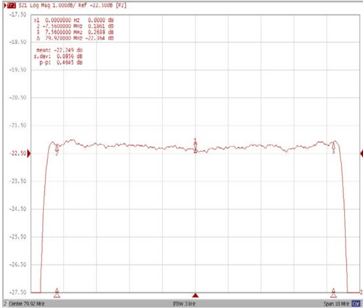
Ripple Variation F_o \pm 7.56\text{MHz}
