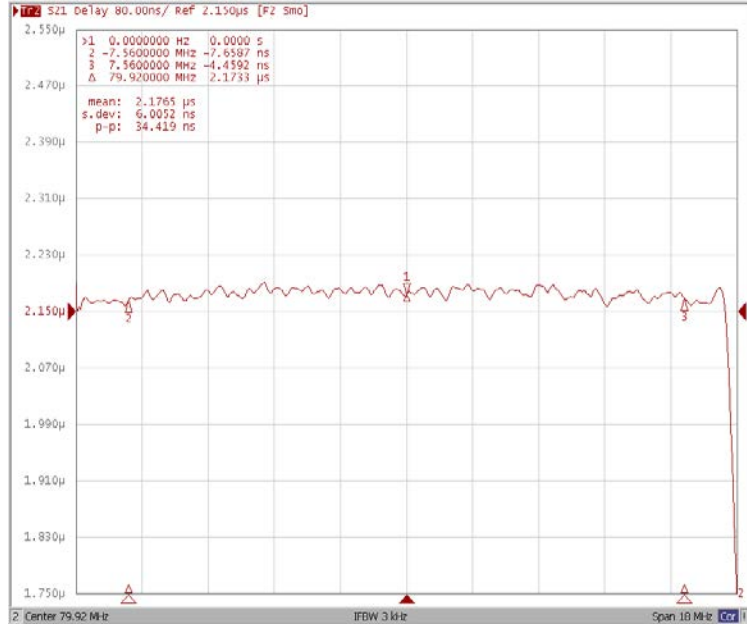
Group Delay Variation F_o \pm 7.56\text{MHz}
