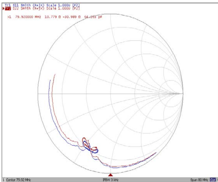
Smith Chart
