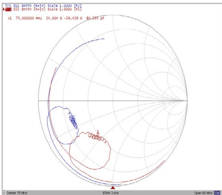
Smith Chart
