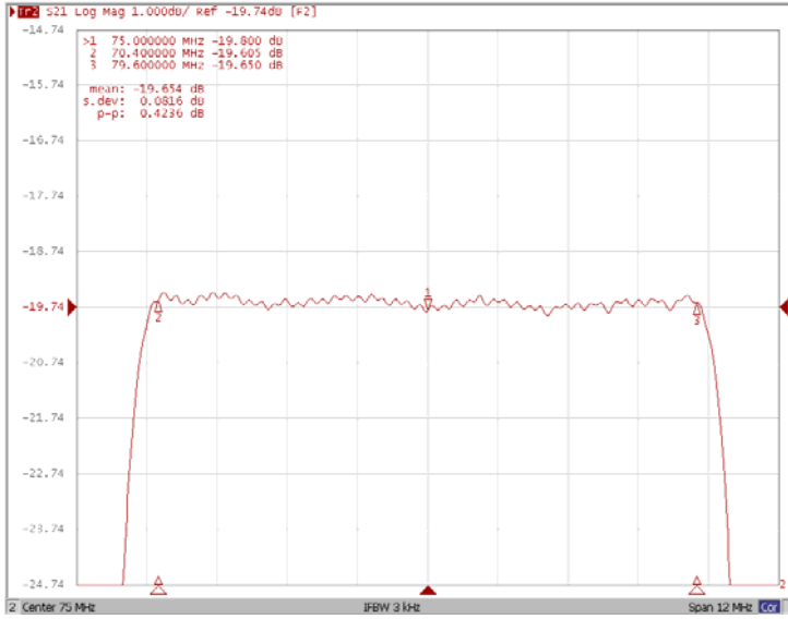
Ripple Variation Fo±4.6MHz
