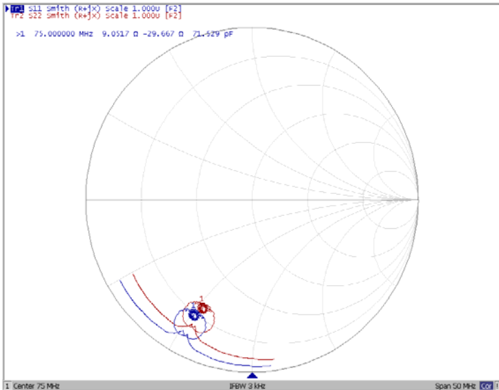
Smith Chart
