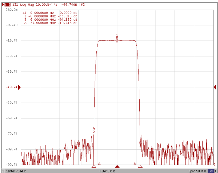
Ultimate Attenuation
