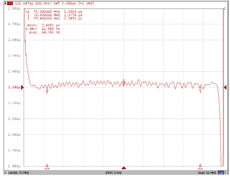
Group Delay Variation Fo±4.6MHz
