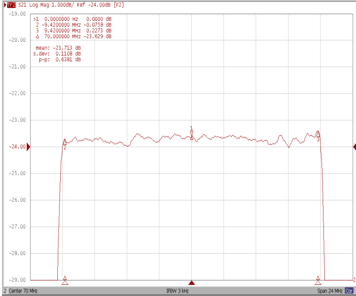
Ripple Variation Fo±9.42MHz
