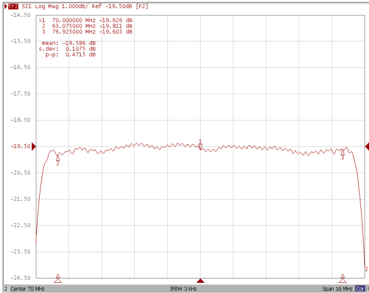
Ripple Variation Fo±6.925MHz
