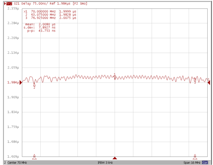
Group Delay Variation Fo±6.925MHz
