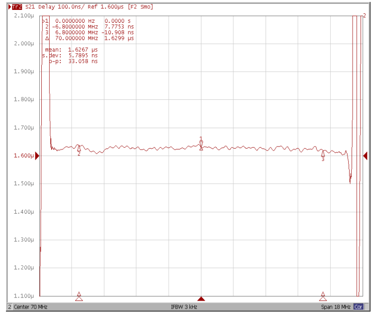
Group Delay Variation Fo±6.8MHz
