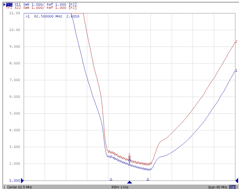
SWR
