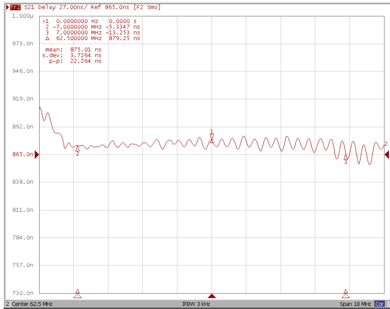
Group Delay Variation at Fo ±7MHz
