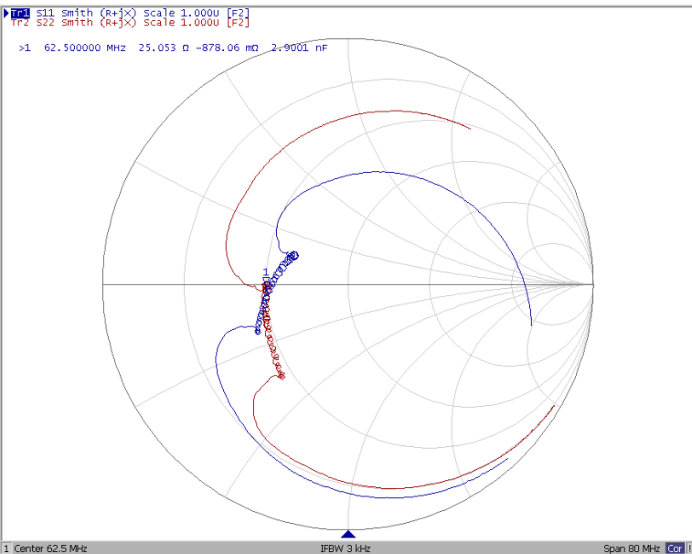
Smith Chart
