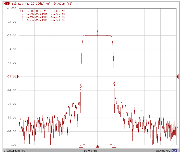
Attenuation Fo ±8.5MHz
