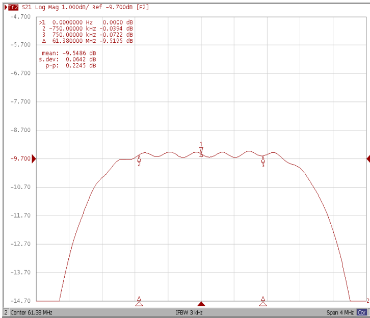
Ripple Variation( F_0 \pm 0.75\text{MHz} )
