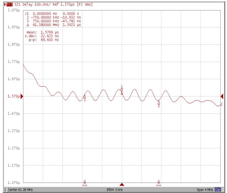
Group Delay Variation( F_0 \pm 0.75\text{MHz} )
