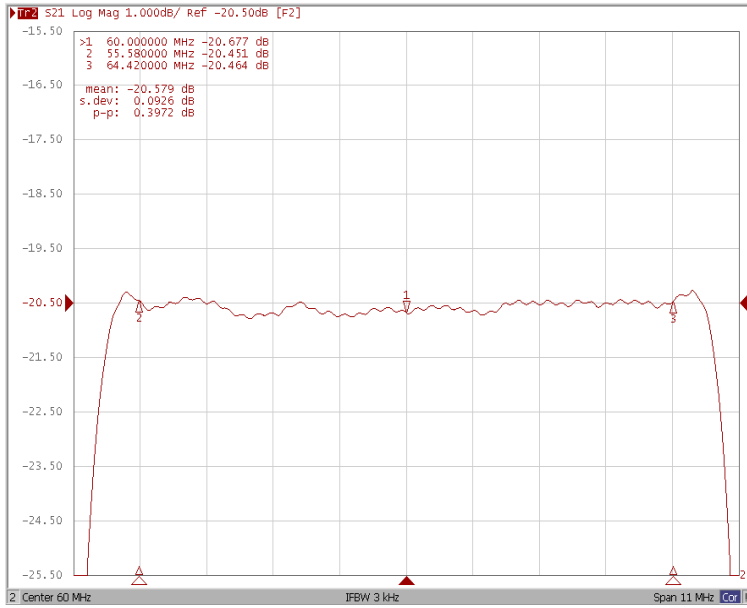
Ripple Variation F_0 \pm 4.42\text{MHz}
