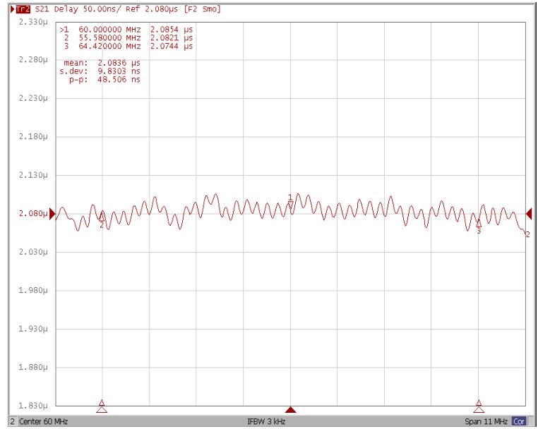
Group Delay Variation F_0 \pm 4.42\text{MHz}
