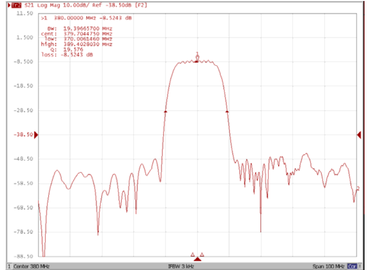
Bandwidth at -20.0 dB
