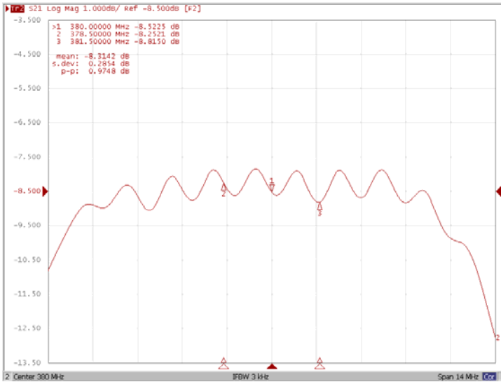
Ripple Variation F_0 \pm 1.5\text{MHz}
