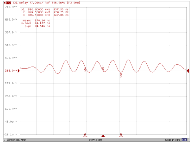
Group Delay Variation F_0 \pm 1.5\text{MHz}
