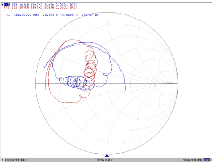
Smith Chart
