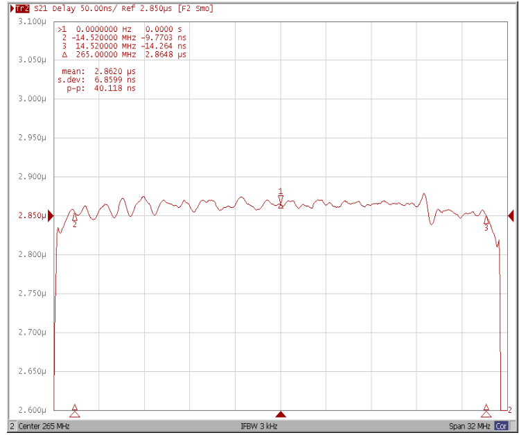
Group Delay Variation F_0 \pm 14.52\text{MHz}
