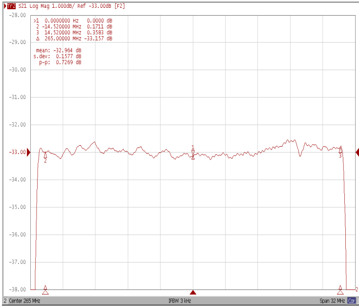
Ripple Variation F_0 \pm 14.52\text{MHz}
