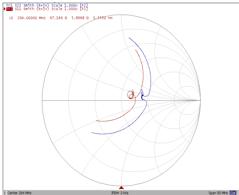
Smith Chart
