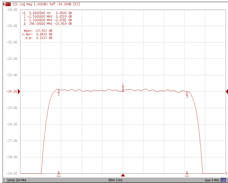
Ripple Variation at Fo±2.5MHz
