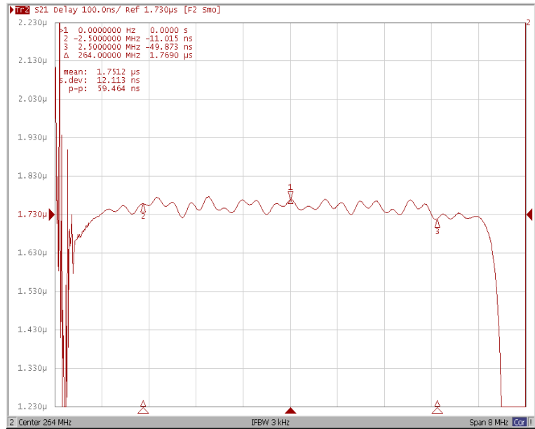
Group Delay Variation at Fo±2.5MHz
