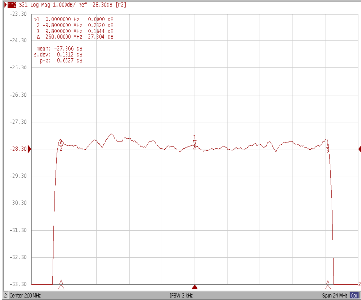
Ripple Variation Fo±9.80MHz
