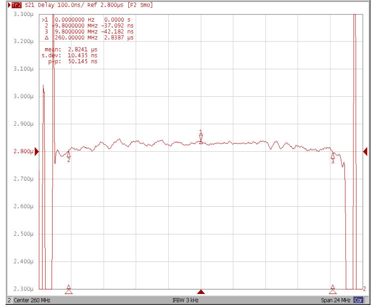
Group Delay Variation Fo±9.80MHz
