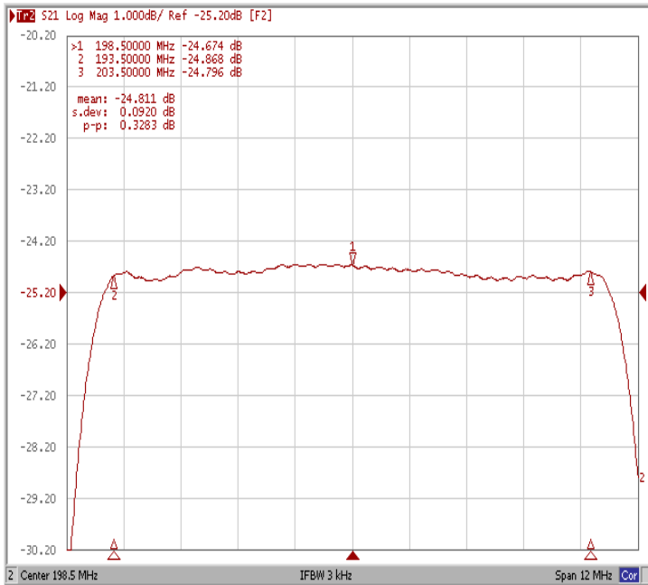
Ripple Variation F_o \pm 5.00\text{MHz}
