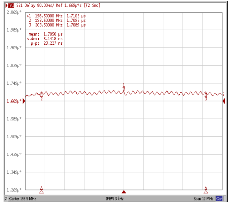
Group Delay Variation F_o \pm 5.00\text{MHz}
