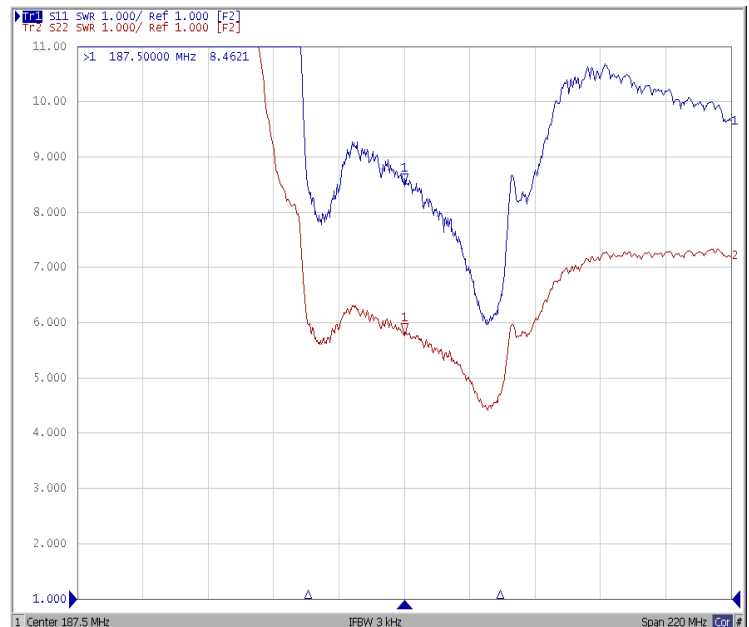
SWR
