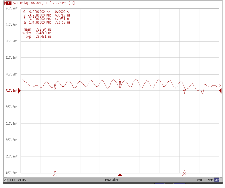
Group Delay Variation Fo±3.9MHz
