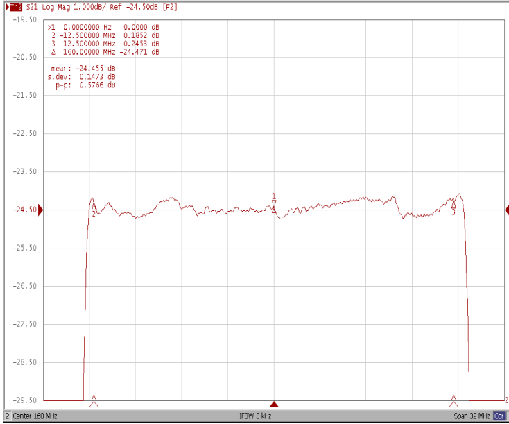
Ripple Variation Fo±12.50MHz
