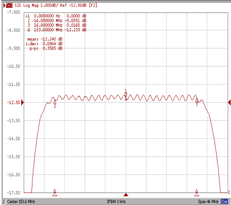
Ripple Variation Fo±16.00MHz
