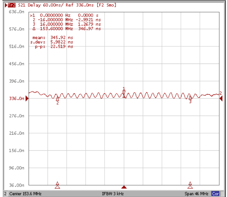
Group Delay Variation Fo±16.00MHz
