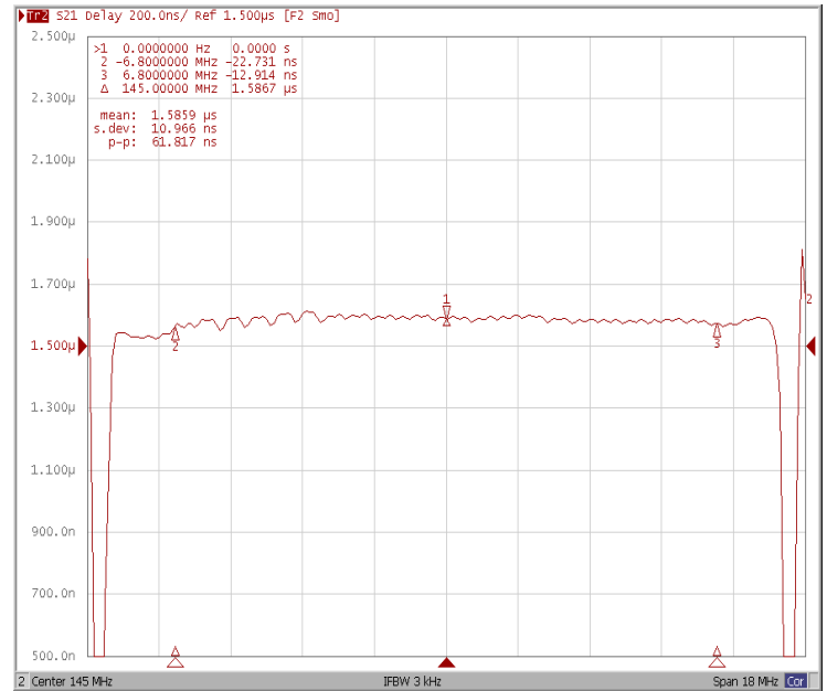
Group Delay Variation
