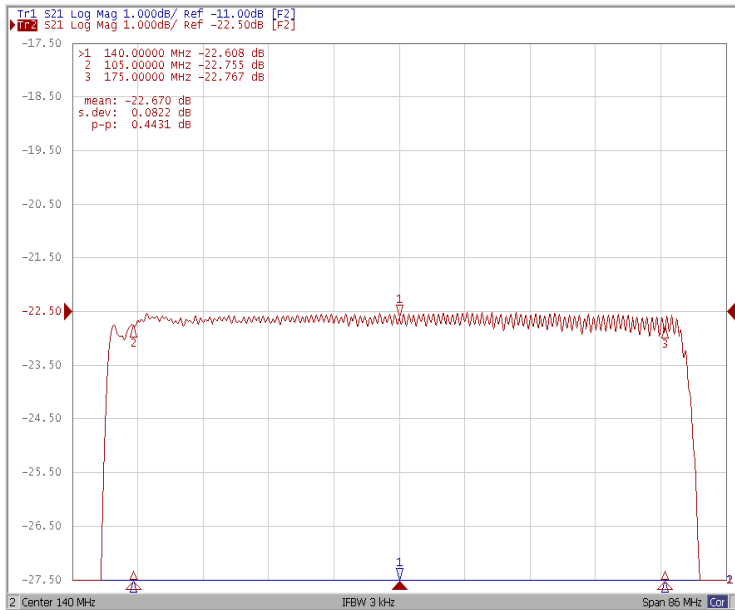
Ripple Variation at F_o \pm 35.0\text{MHz}
