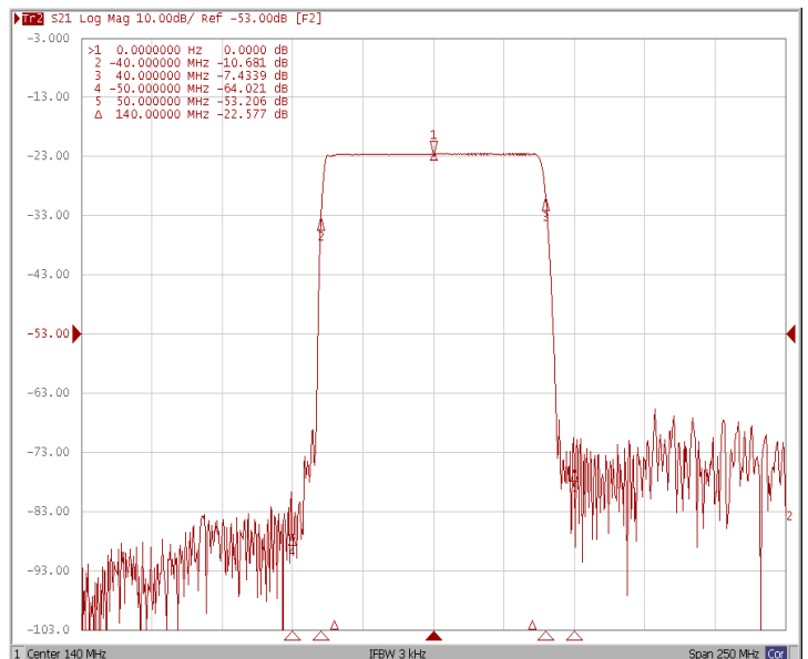
Relative Attenuation at Fo±40.0MHz , ±50.0MHz
