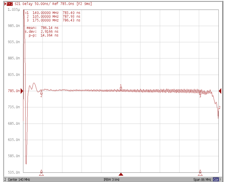
Group Delay Variation at F_o \pm 35.0\text{MHz}
