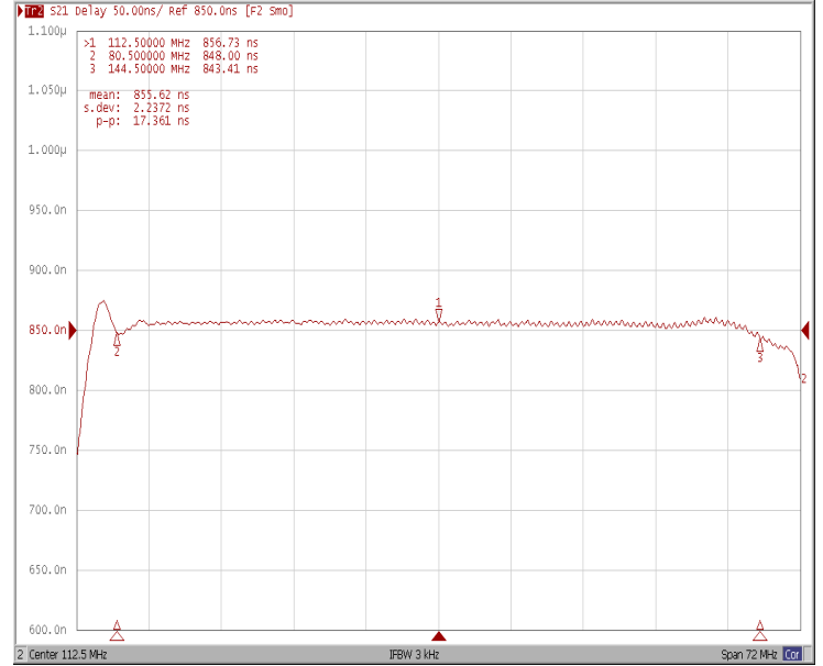
Group Delay Variation Fo±32.0MHz
