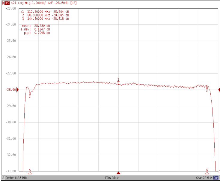
Ripple Variation Fo±32.0MHz
