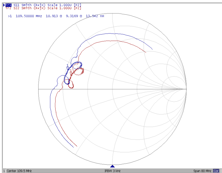
Smith Chart
