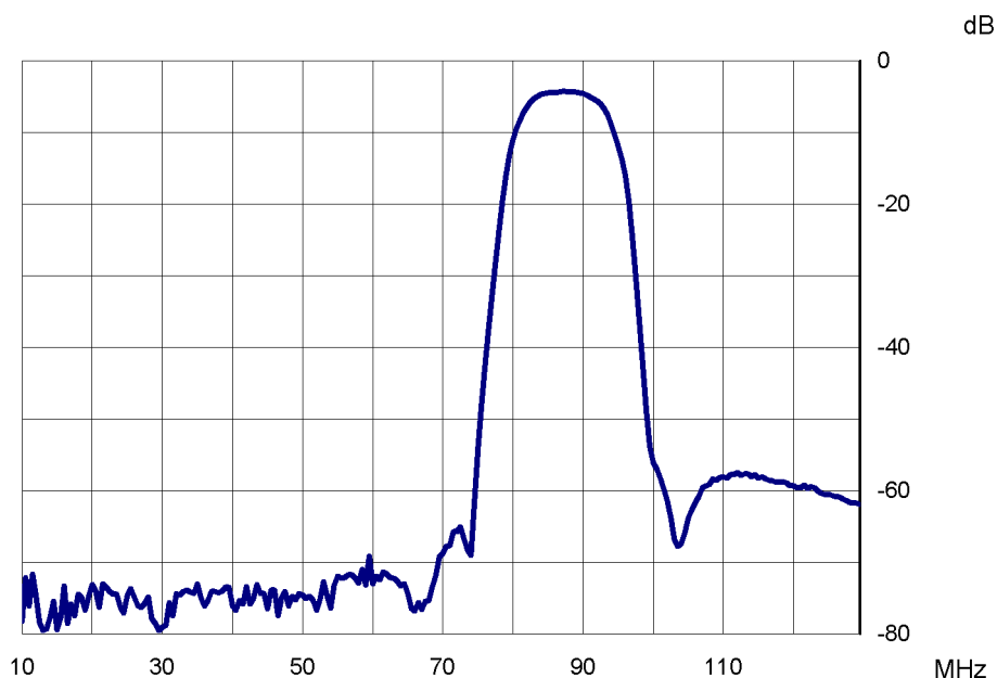
Amplitude-frequency response
