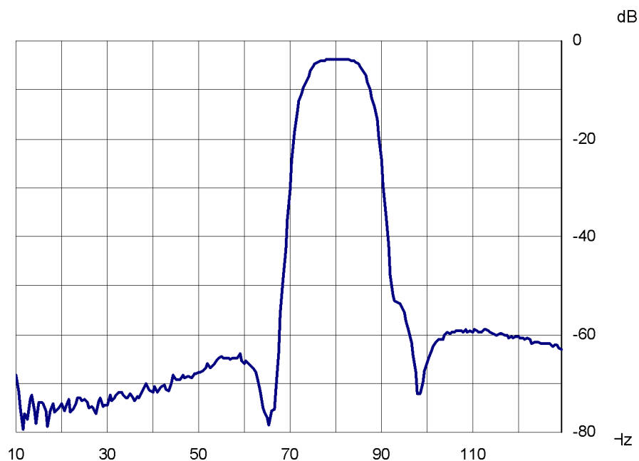
Amplitude-frequency response
